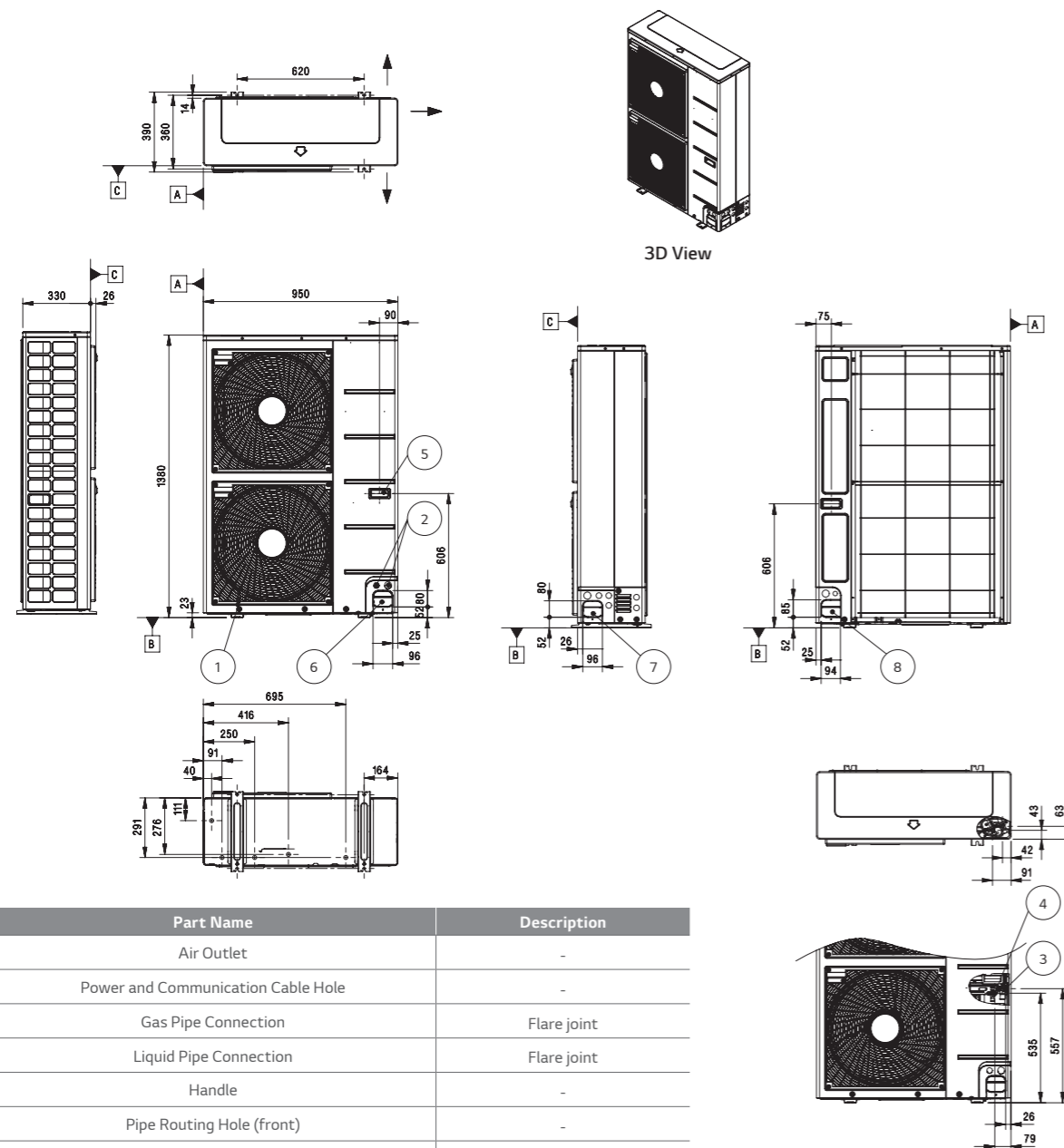
Piping Connection Port
